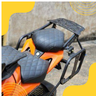
TOP RACK AND SADDLE STAY KTM RC 200 & 390 BS6 HI TECH
